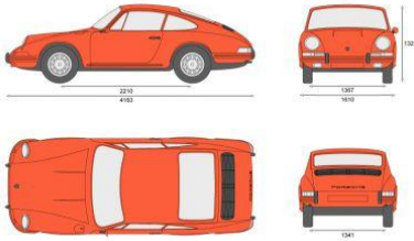
Porsche 911 S (1963)
