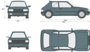
Peugeot 205 Turbo 16 (1985)
