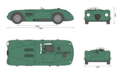
Jaguar C-Type (1951)
