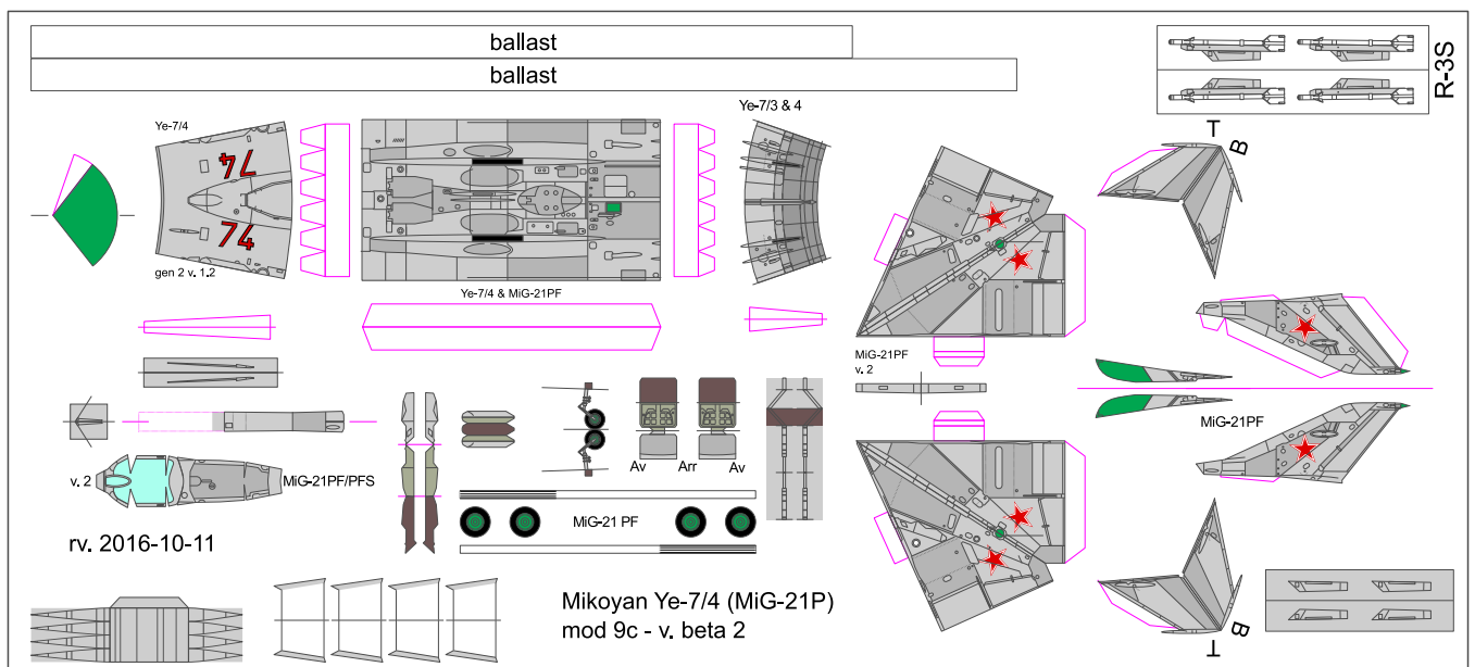
Mikoyan Ye-7/4 (MiG-21P) early configuration
